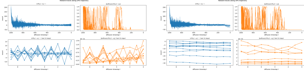
Figure 4: We plot a projected discrepancy (f(x_t) - \mathbb{1}_k) \cdot \mathbb{1} ((Columns 1 and 3)) and the reward \|f(x_t) - \mathbb{1}_k\| ((Columns 2 and 4)) across t where denoising proceeds from left (most noise) to right (least noise). The second row depicts a close-up plot of just the last 10 steps to highlight the oscillations. (Columns 1 and 2) are run with a constant guidance schedule Algorithm 1, while (Column 3 and 4) are run with early guidance stopping Algorithm 2 with parameter i_{stop} = 100 .
