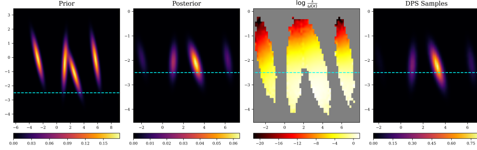
Figure 2: True Posterior versus DPS Samples: Dashed line is measurement constraint Ax = y , A(x_1, x_2) = (0, x_2) , y = (0, -2.5) . (a) Prior (analytic): \rho_0 , 4-component, equal-weight, Gaussian mixture; (b) Posterior (analytic): \mu^y = \frac{\exp(R)}{Z} \rho_0 where R(x_1, x_2) = -2 \|Ax - y\|^2 ; (c) Weight (log-scale): \frac{1}{\omega(x)} , 20 trajectory estimate, darkest is undersampling, lightest is oversampling, gray background not computed; (d) DPS Samples: 5 \times 10^5 samples show x_1 -extremal modes are nearly absent while x_2 < y_2 is over-sampled and x_2 > y_2 undersampled.
