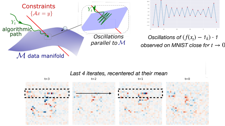
Figure 3: (Top Left) A pictorial depiction of instability - as the trajectory approaches the data manifold, the large effective guidance schedule triggers oscillations in the trajectory. (Top Right) An exhibition of these oscillation on a posterior sampling task with an MNIST prior. (Bottom) A plot of the last four iterates of DPS, re-centered about their mean. The guidance tilted the distribution towards the digit 3. We observe periodic oscillations in pixel space (the deviations from the mean at alternate time steps are similar to each other). Please see Figure 4 and Appendix H for details.
