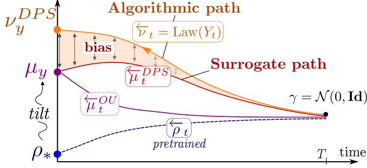
Figure 1: The blue dotted line illustrates the path taken by the standard forward OU process from \rho_* , \vec{\rho}_t and its reversal \overleftarrow{\rho}_t . The violet line illustrates the OU process \overleftarrow{\mu}_t^{OU} , whose reversal \overrightarrow{\mu}_t we cannot track at inference time. The red line illustrates the surrogate path \overrightarrow{\mu}_t^{DPS} = e^{R_y(\hat{x}_t)} \rho_*/Z we construct, with the same beginning and end points as \vec{\mu}_t . The orange line denotes the algorithm path \nu_t^{DPS} which disregards the reaction term results in a sample from \nu_y^{DPS} with an unavoidable bias.
