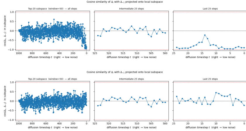
Figure 5: Top Are plots associated to the standard DPS algorithm Algorithm 1, Top Left We plot \alpha_t = (\mathcal{P}_t^k \delta_t) \cdot (\mathcal{P}_t^k \delta_{t-1}) along the DPS trajectories for a constant guidance schedule \zeta = 0.1 . Top Middle A close-up of steps 525 \rightarrow 500. Top Right A close-up of steps 25 \rightarrow 0. Note that \alpha_t is close to 0 at the intermediate noise levels, but drops to \approx -1 towards the low noise levels. Bottom Are the same plots associated to Algorithm 2 with i_{stop} = 100 . We observe that \alpha_t remains close to 0 both at intermediate noise levels and low noise levels.
